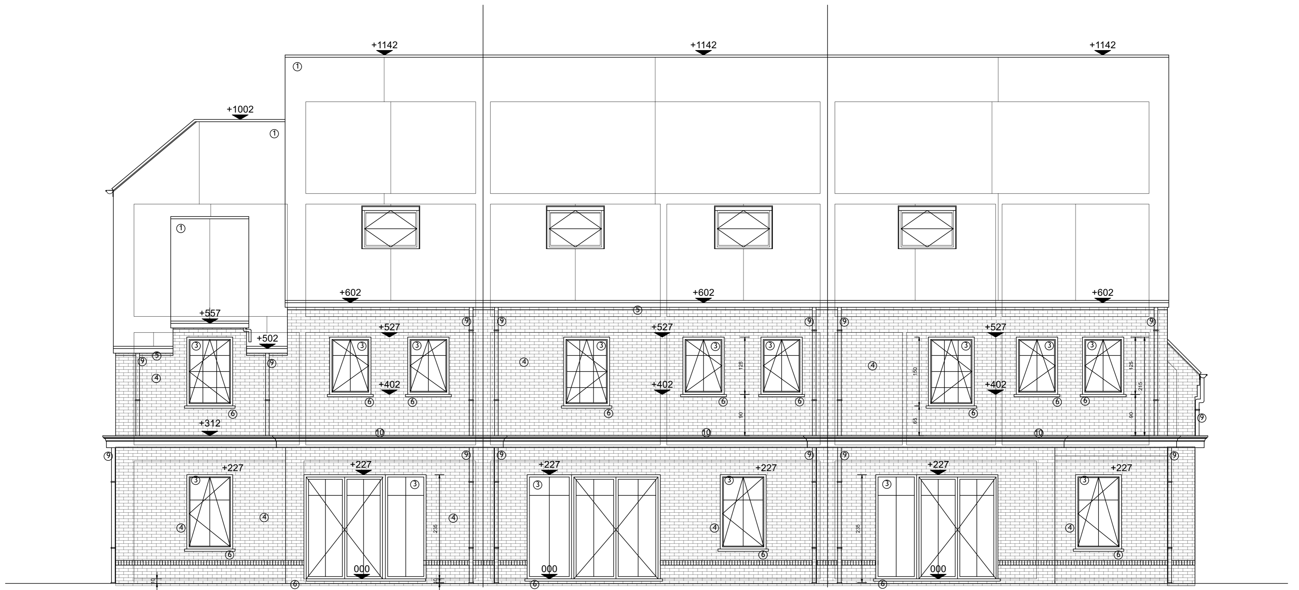
ACHTERGEVEL, LOT 3, LOT 2, LOT 1 SCHAAL 1/50
